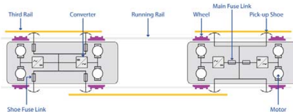
Figure 3: Fusing Options
