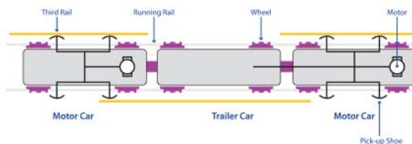
Figure 2: Typical Shoe and Power Arrangement (sub surface)
