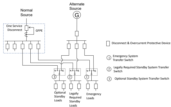
Figure 6 Normal source service at 480/277 V and service disconnect 1000 A or greater having GFPE per 230.95.
