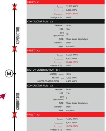
Documentation for available fault current and calculation date - example via Bussmann series FC 2 Available Fault Current Calculator.
