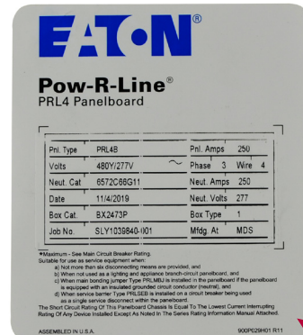
Figure 12 Eaton PRL-4 panelboard label providing advisement on how to determine the assembly SCCR.
