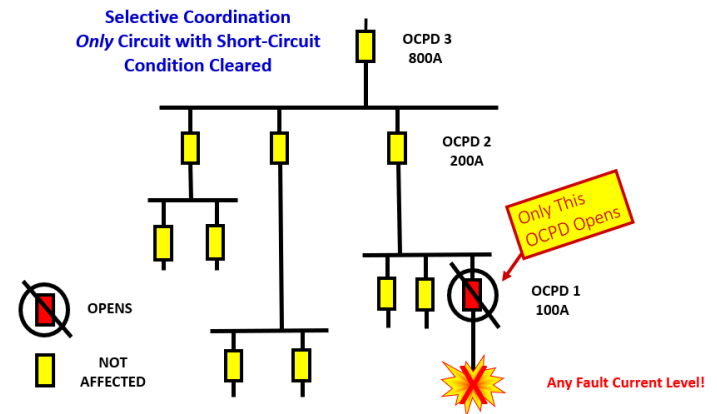
Figure 1. In this example, selective coordination means if a fault occurs on the load side of OCPD 1 (100 A), only that OCPD opens. Neither OCPD 2 (200 A) nor OCPD 3 (800 A) opens. Selective coordination also means this principle is valid for the full range of overcurrents including the available fault currents throughout the system being analyzed.
