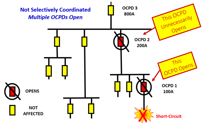
Figure 2. Example of non-selective coordination: for some range of fault currents, a fault as shown causes OCPD 1 to clear the circuit as intended. However, due to a lack of selective coordination, OCPD 2 unnecessarily opens, which results in some loads unnecessarily being interrupted. OCPD 3 might also unnecessarily open due to lack of selective coordination and this would result in the entire system being without power.
