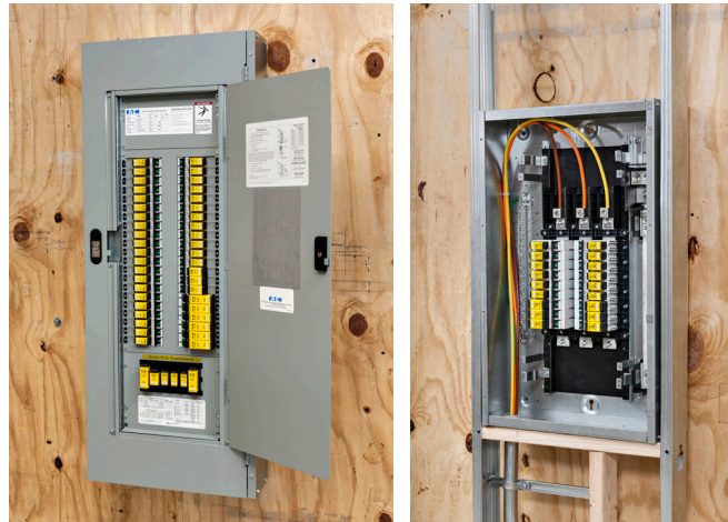
The Bussmann series Quik-Spec Coordination Panelboard with current-limiting Class CF CUBEFuse overcurrent protection.
