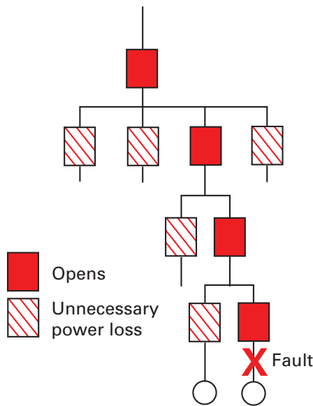
Without selective coordination
