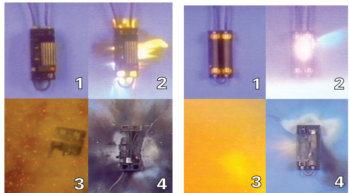
A circuit breaker misapplied beyond its interrupting rating.
