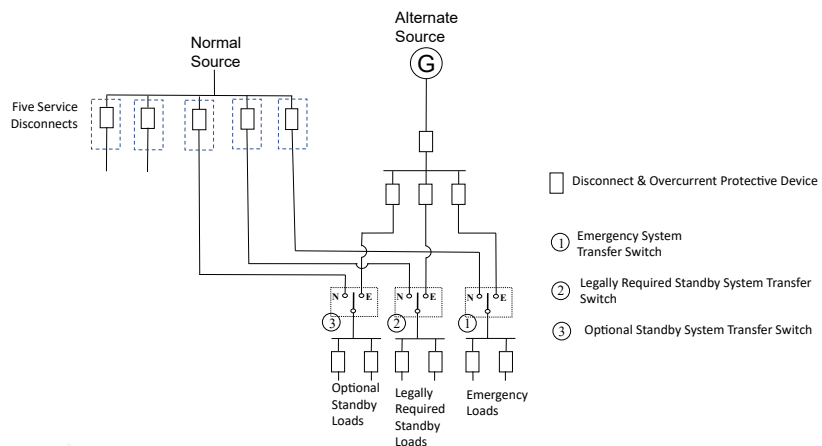
Figure 8 If the normal source disconnects to the emergency system and legally required standby system are less than 1000 A, as well as the other normal source disconnects, the 230.71(B) two to six service disconnect rule permits this configuration without GFPE. (480/277 V system)
