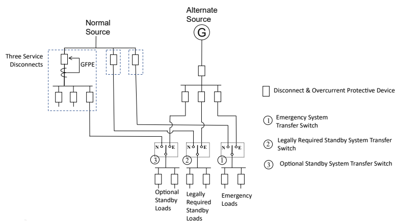
Figure 7 If the normal source disconnects to the emergency system and legally required standby system are less than 1000 A, the 230.71(B) two to six service disconnect rule permits this configuration with GFPE. (480/277 V system)
