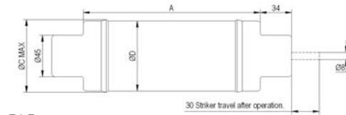
EJ Fuses
