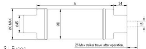
SJ Fuses
