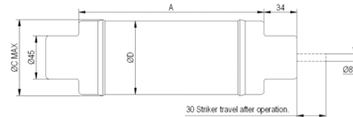
EJ Fuses
